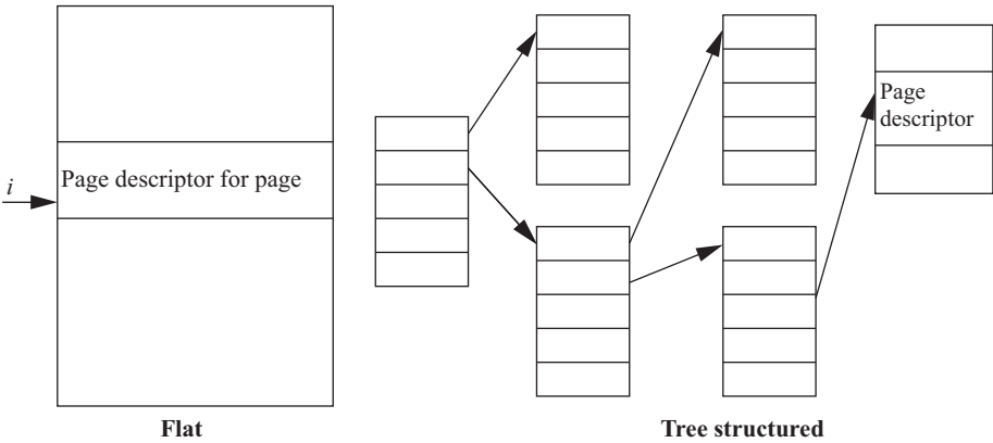
FIGURE 3.14 Alternative schemes for organizing page tables.
