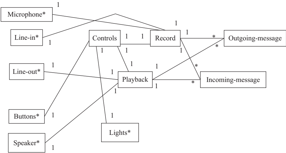
FIGURE 6.21 Class diagram for the answering machine.
