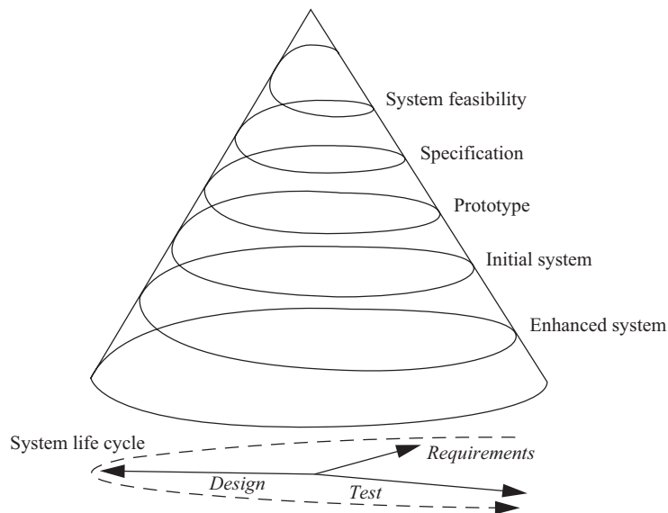
FIGURE 7.2 The spiral model of software design.
