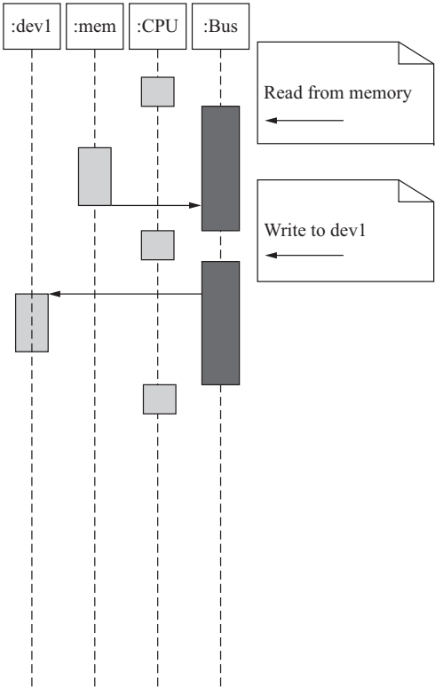
FIGURE 4.5 A typical sequence diagram for bus operations.
