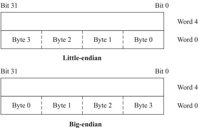
FIGURE 2.7 Byte organizations within an ARM word.
