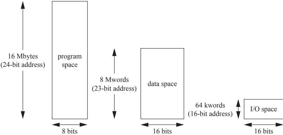
FIGURE 2.22 Address spaces in the TMS320C55x.
