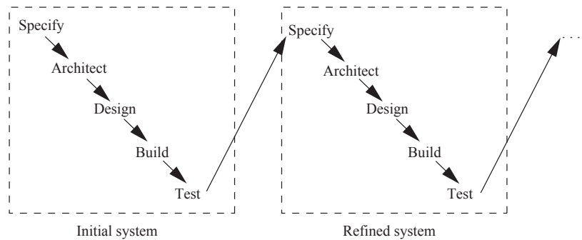
FIGURE 7.3 A successive refinement development model.
