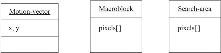
FIGURE 10.20 Classes describing basic data types in the video accelerator.
