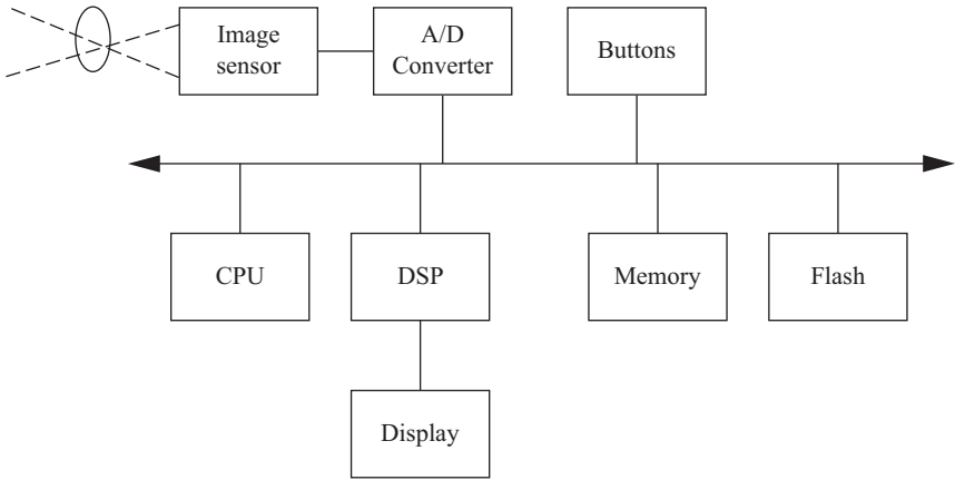
FIGURE 5.42 Computing platform for a digital still camera.
