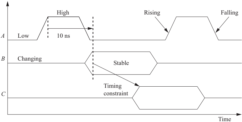
FIGURE 4.6 Timing diagram notation.
