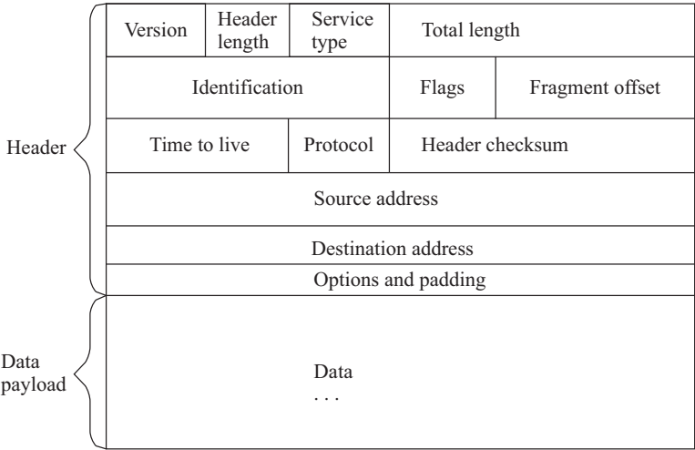
FIGURE 8.6 IP packet structure.
