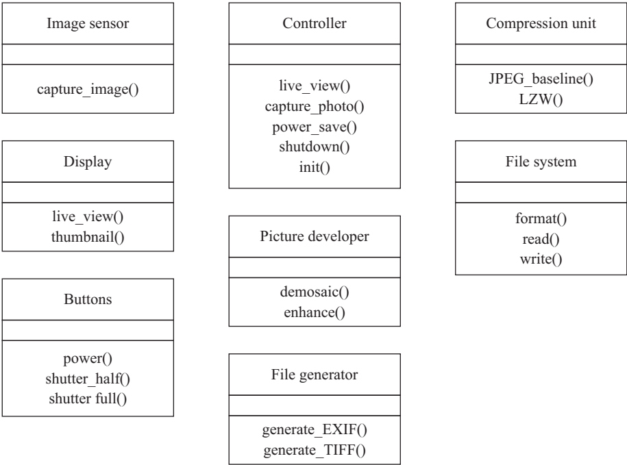
FIGURE 5.41 Basic classes in the digital still camera.
