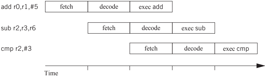
FIGURE 3.16 Pipelined execution of ARM instructions.
