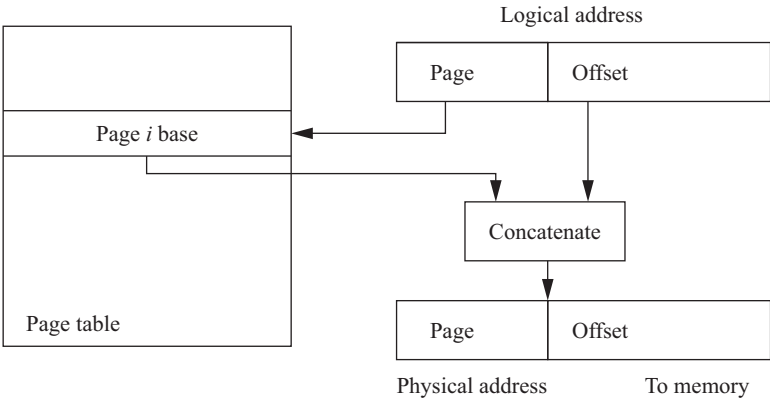
FIGURE 3.13 Address translation for a page.
