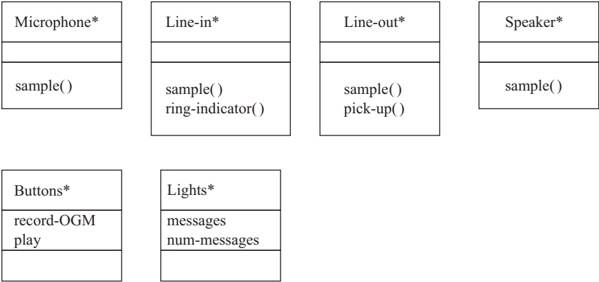
FIGURE 6.22 Physical class interfaces for the answering machine.
