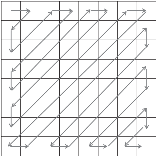
FIGURE 5.36 Zig-zag pattern for reading coefficients.
