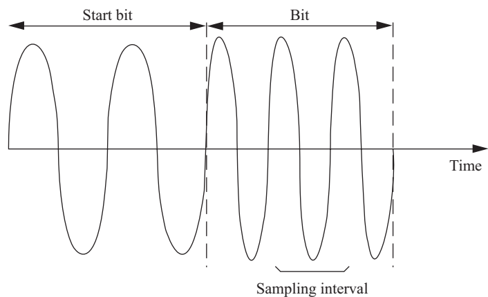
FIGURE 5.31 Receiving bits in the modem.
