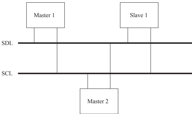
FIGURE 10.10 Structure of an I 2 C bus system.
